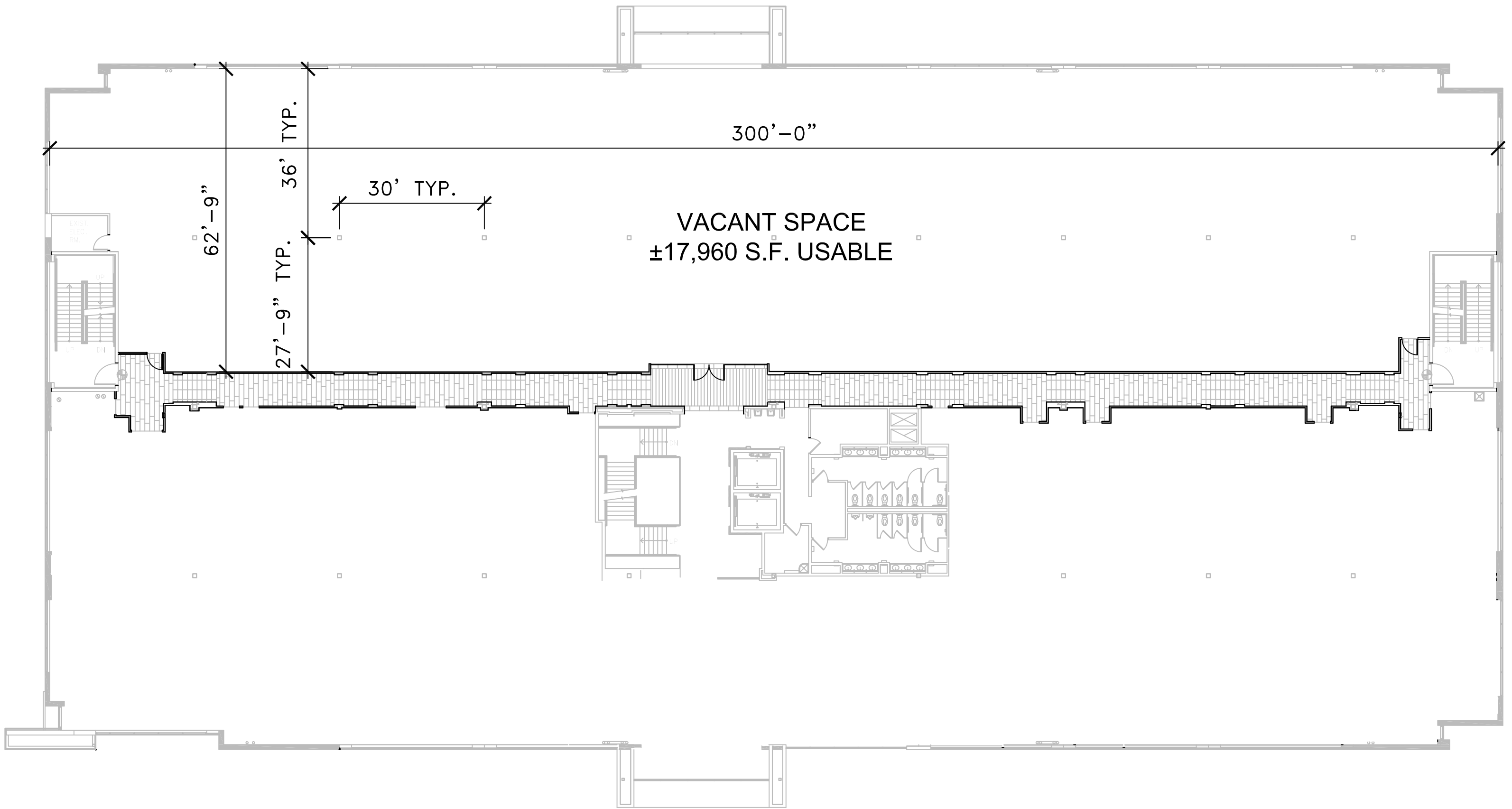
CAZ 5 BUILDING 1 2ND FLOOR NOT TO A SPECIFIC SCALE
